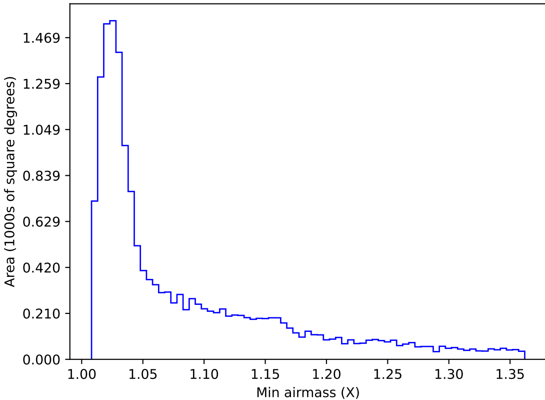
baseline_v3.0_10yrs WFD g band: Min airmass
