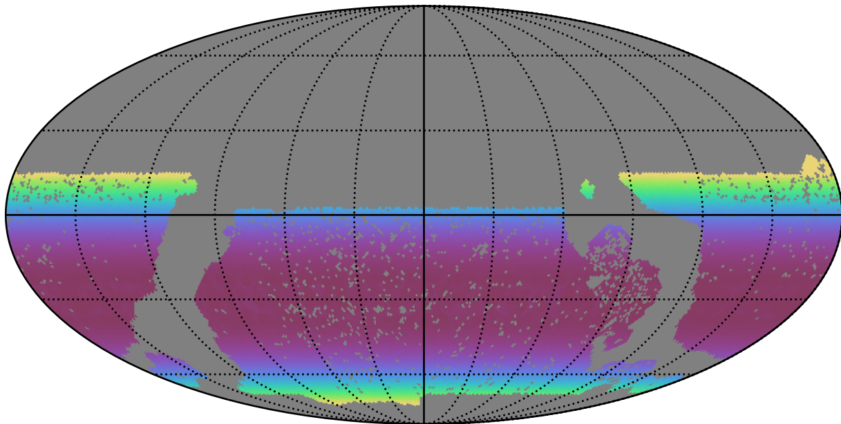
baseline_v3.0_10yrs WFD all bands: Min airmass
