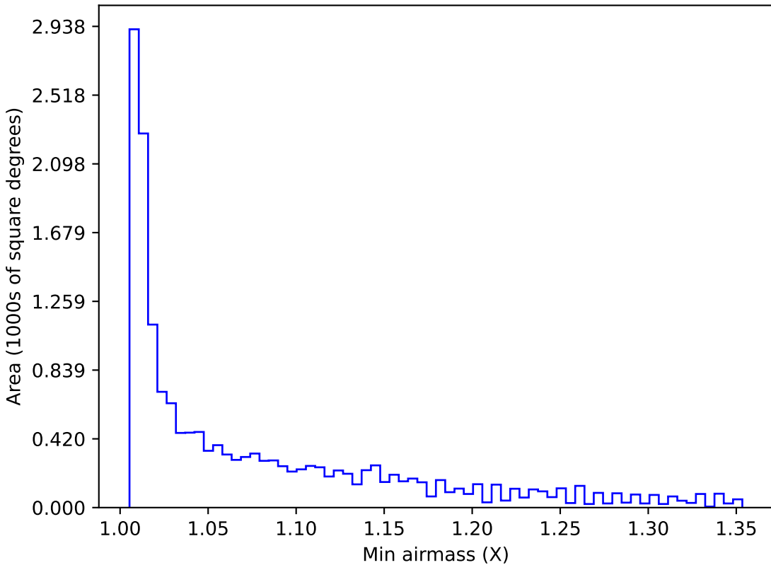
baseline_v3.0_10yrs WFD all bands: Min airmass
