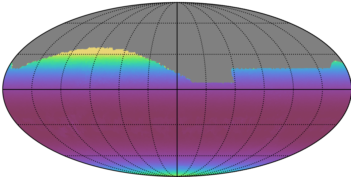
baseline_v3.0_10yrs All sky z band: Min airmass
