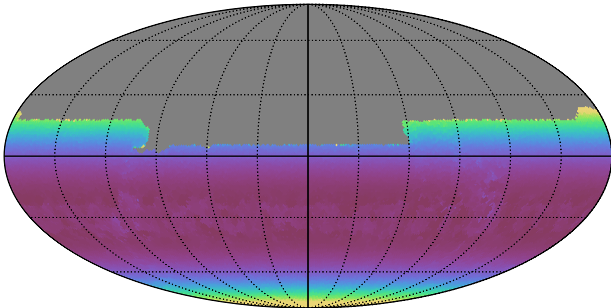
baseline_v3.0_10yrs All sky u band: Min airmass
