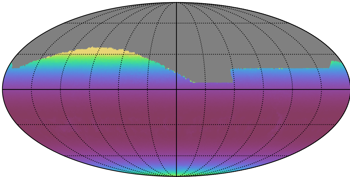
baseline_v3.0_10yrs All sky r band: Min airmass
