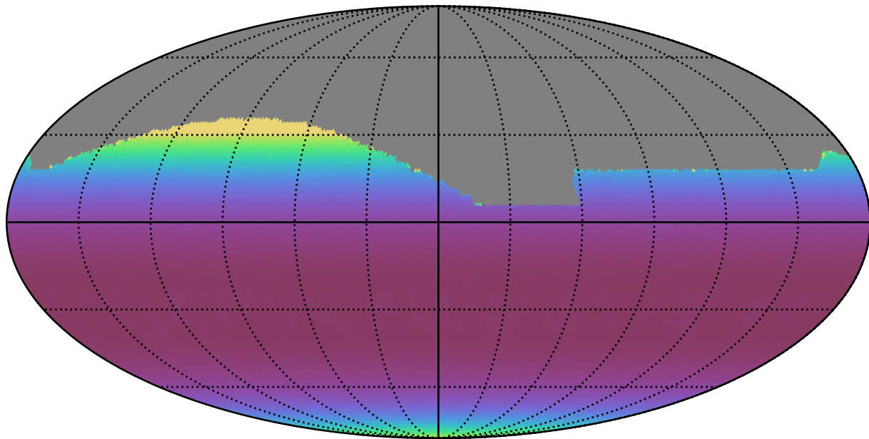
baseline_v3.0_10yrs All sky i band: Min airmass
