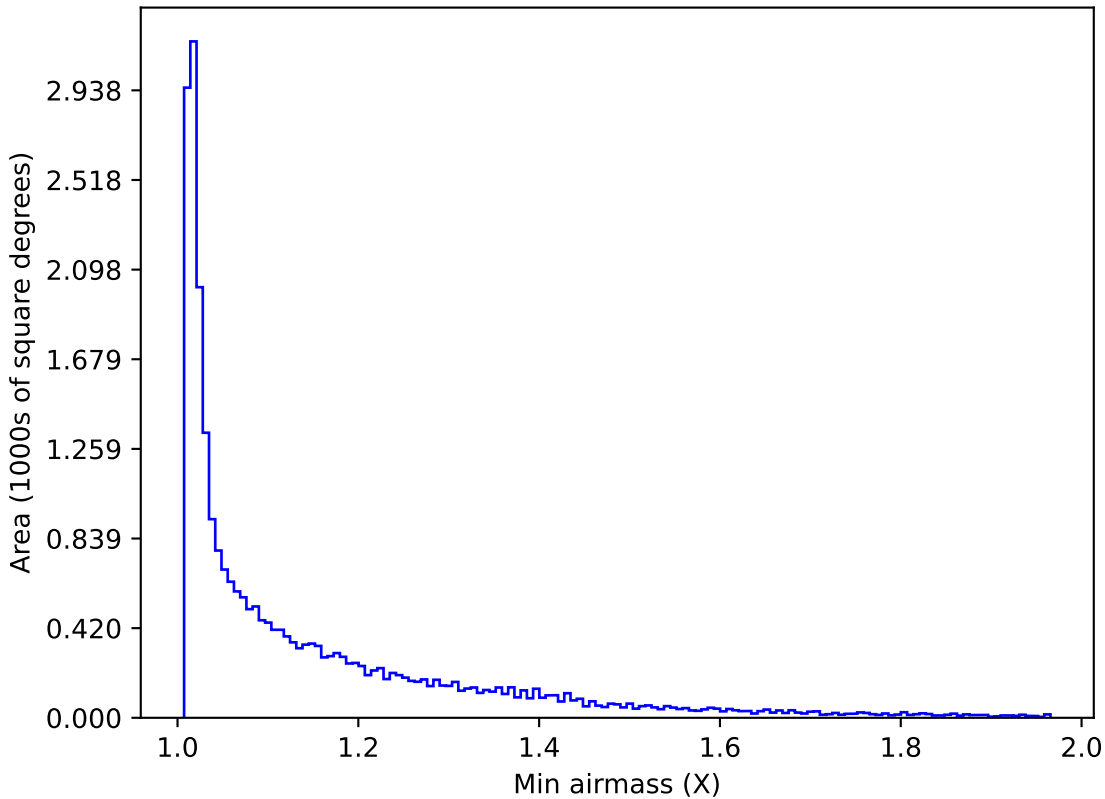
baseline_v3.0_10yrs All sky i band: Min airmass
