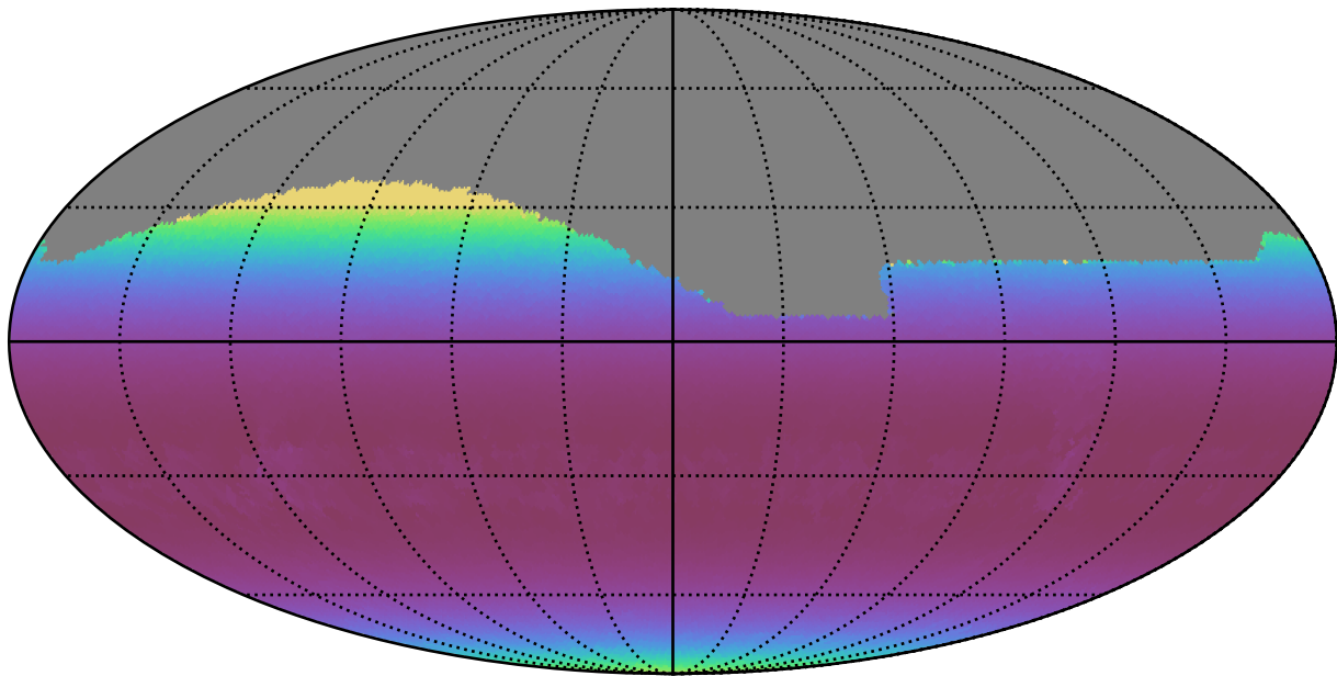
baseline_v3.0_10yrs All sky g band: Min airmass
