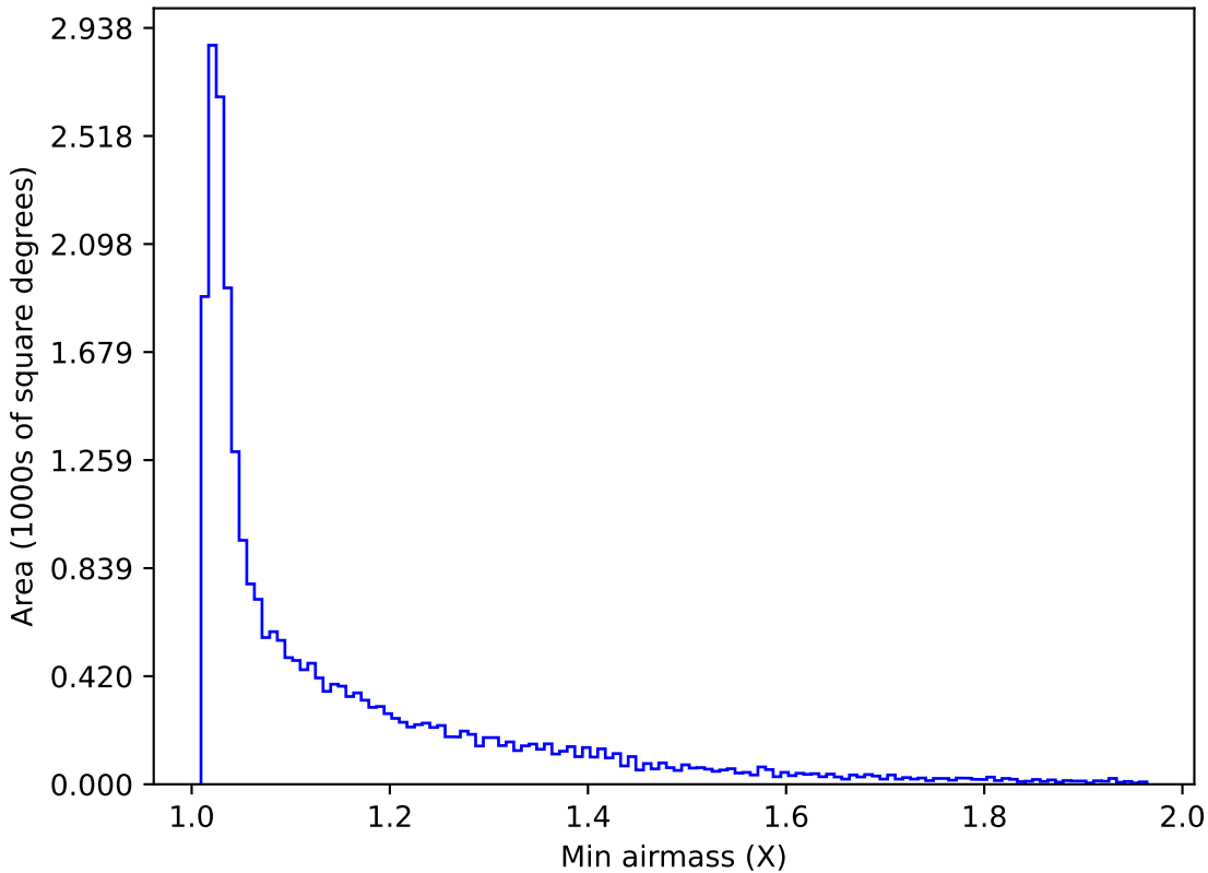
baseline_v3.0_10yrs All sky g band: Min airmass
