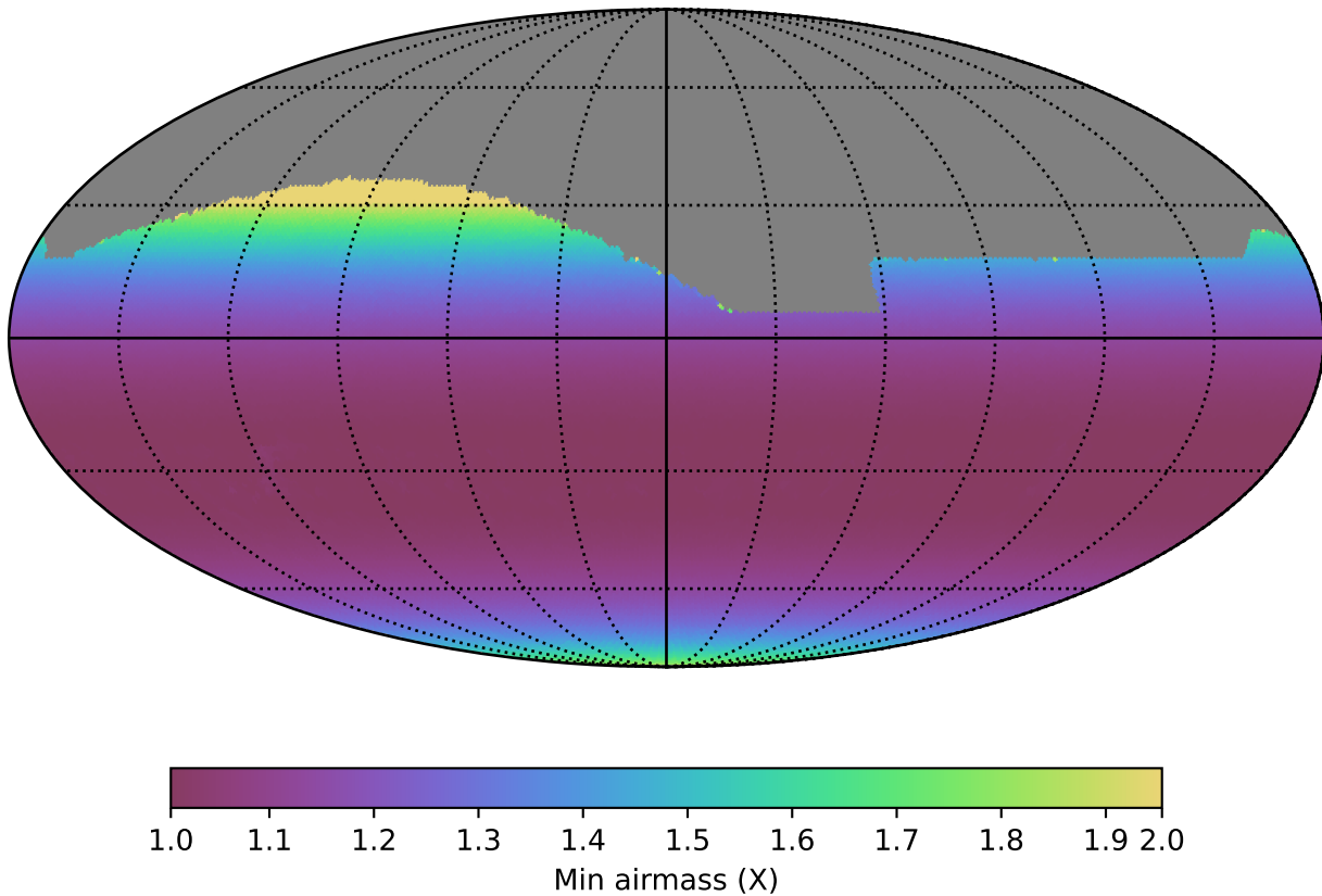
baseline_v3.0_10yrs All sky all bands: Min airmass
