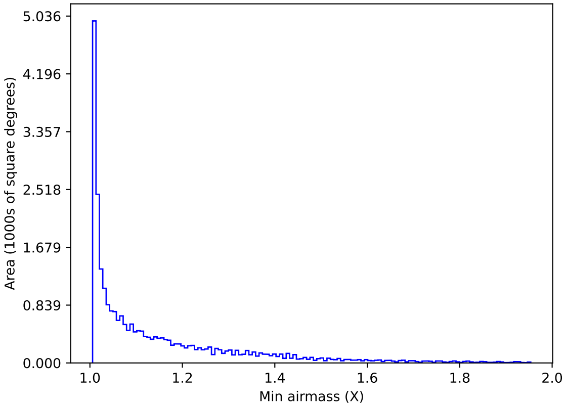
baseline_v3.0_10yrs All sky all bands: Min airmass
