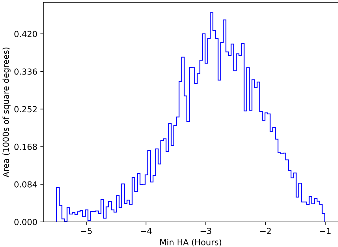
baseline_v3.0_10yrs WFD u band: Min HA
