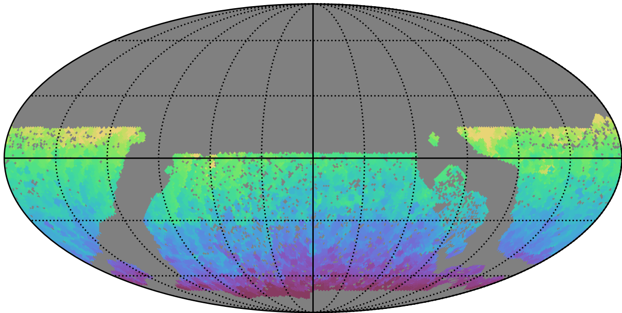
baseline_v3.0_10yrs WFD all bands: Min HA
