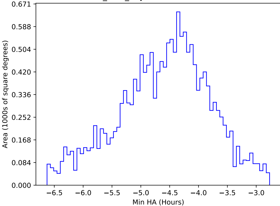
baseline_v3.0_10yrs WFD all bands: Min HA
