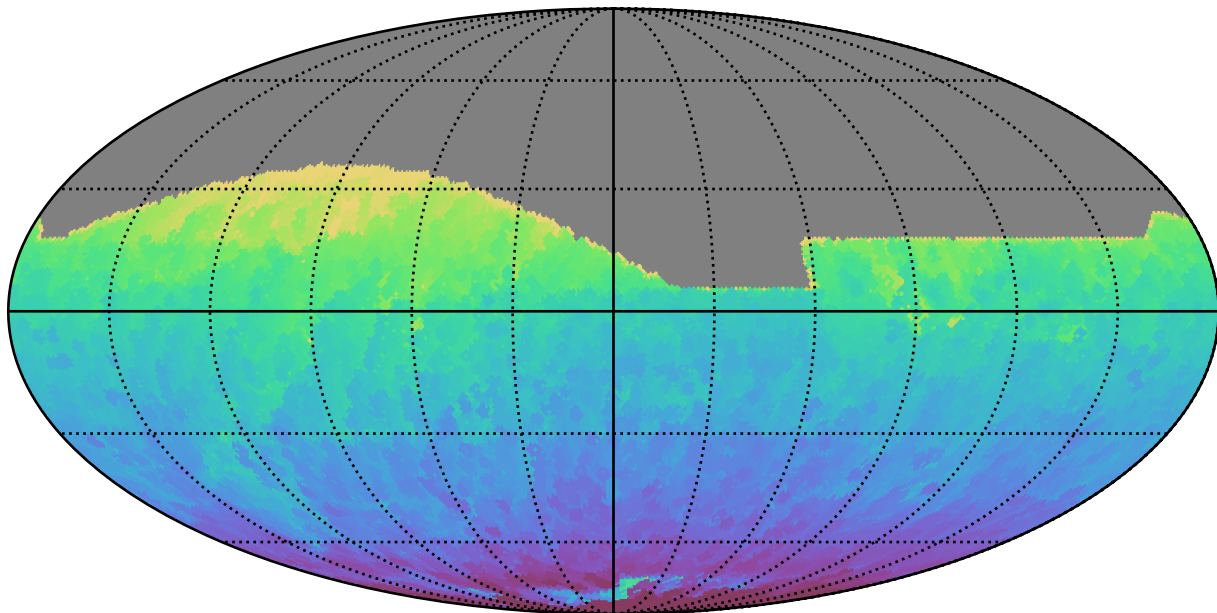
baseline_v3.0_10yrs All sky all bands: Min HA
