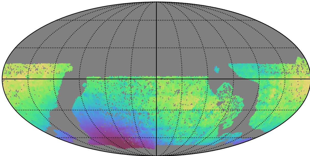
baseline_v3.0_10yrs WFD z band: Median solarElong
