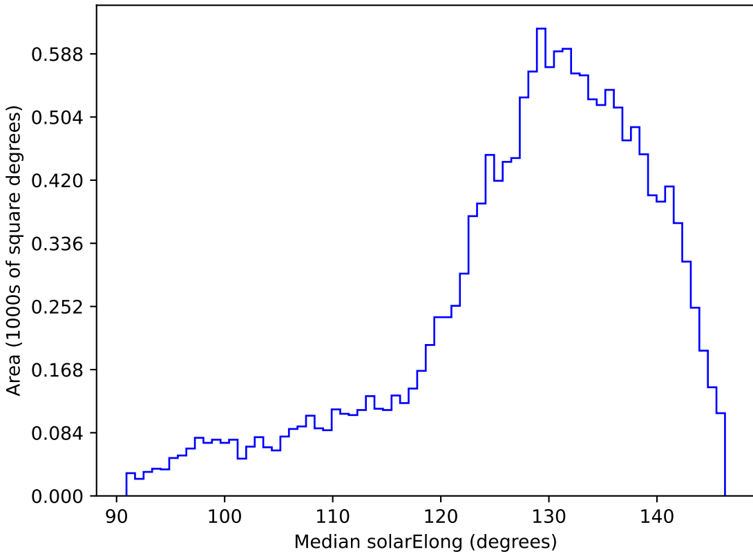
baseline_v3.0_10yrs WFD z band: Median solarElong
