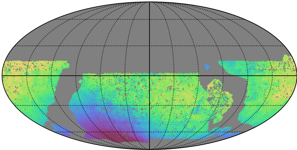
baseline_v3.0_10yrs WFD y band: Median solarElong
