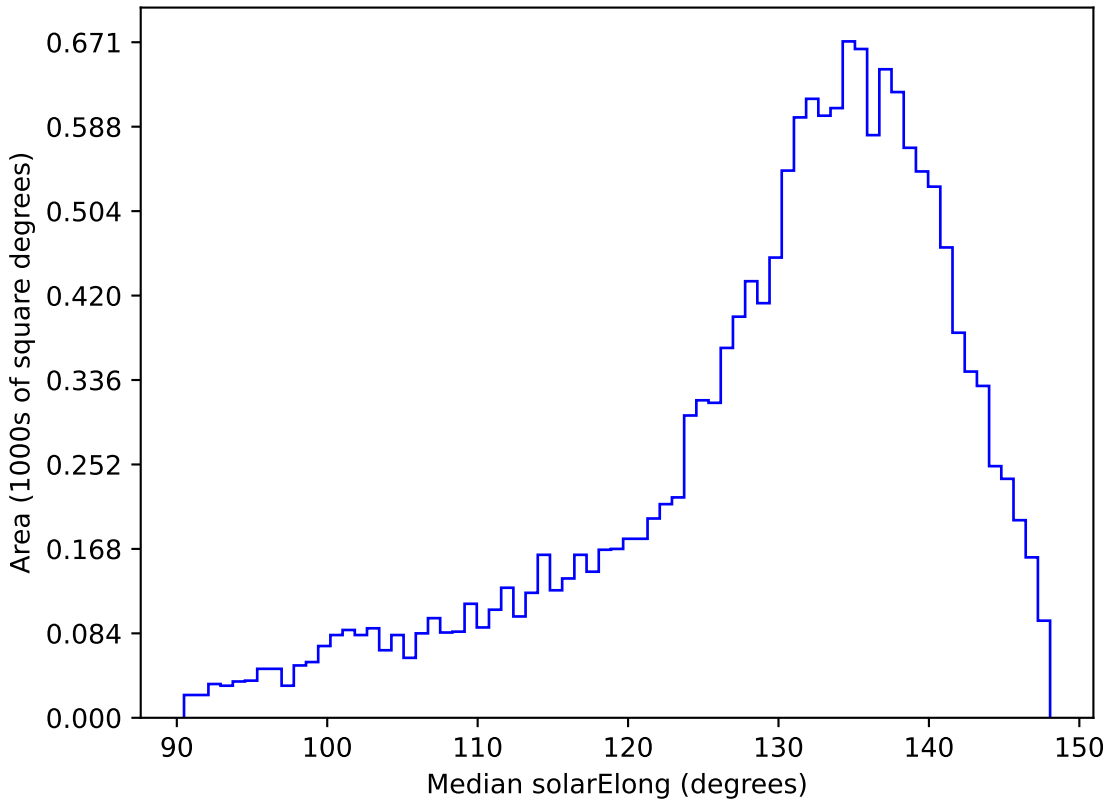
baseline_v3.0_10yrs WFD y band: Median solarElong
