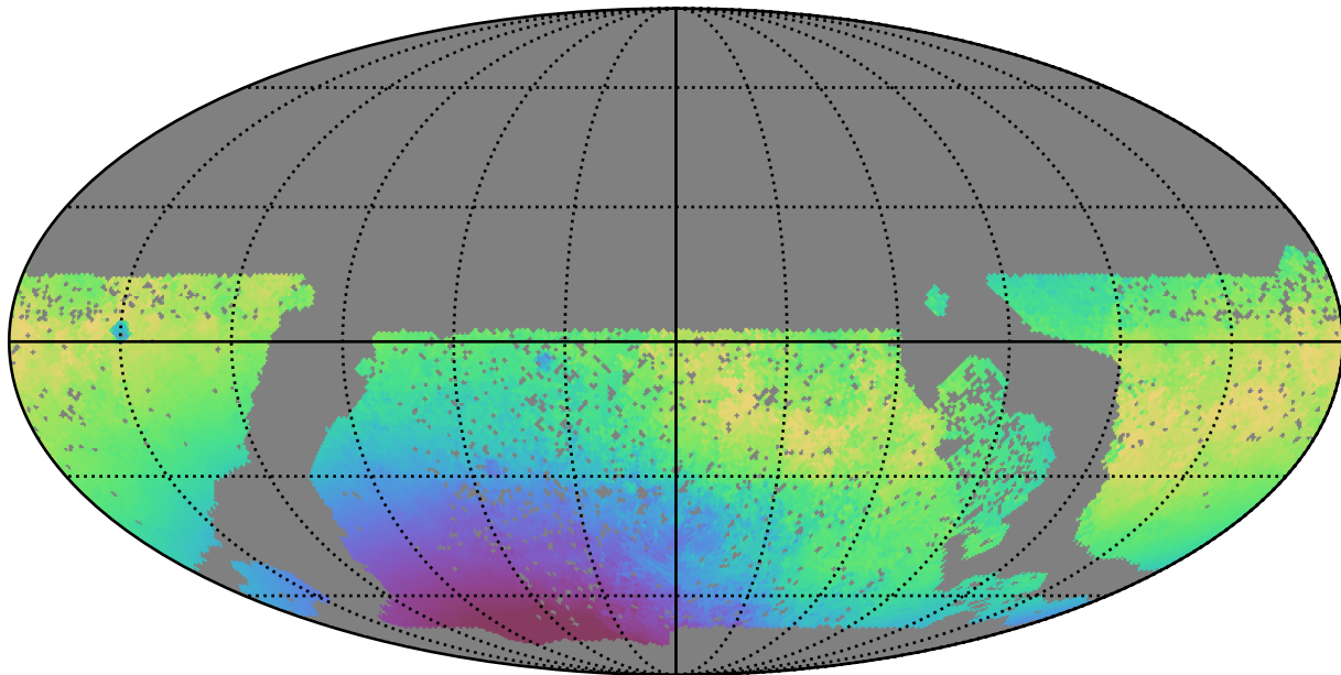
baseline_v3.0_10yrs WFD u band: Median solarElong
