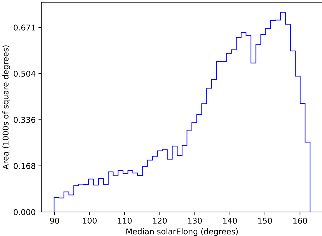
baseline_v3.0_10yrs WFD u band: Median solarElong
