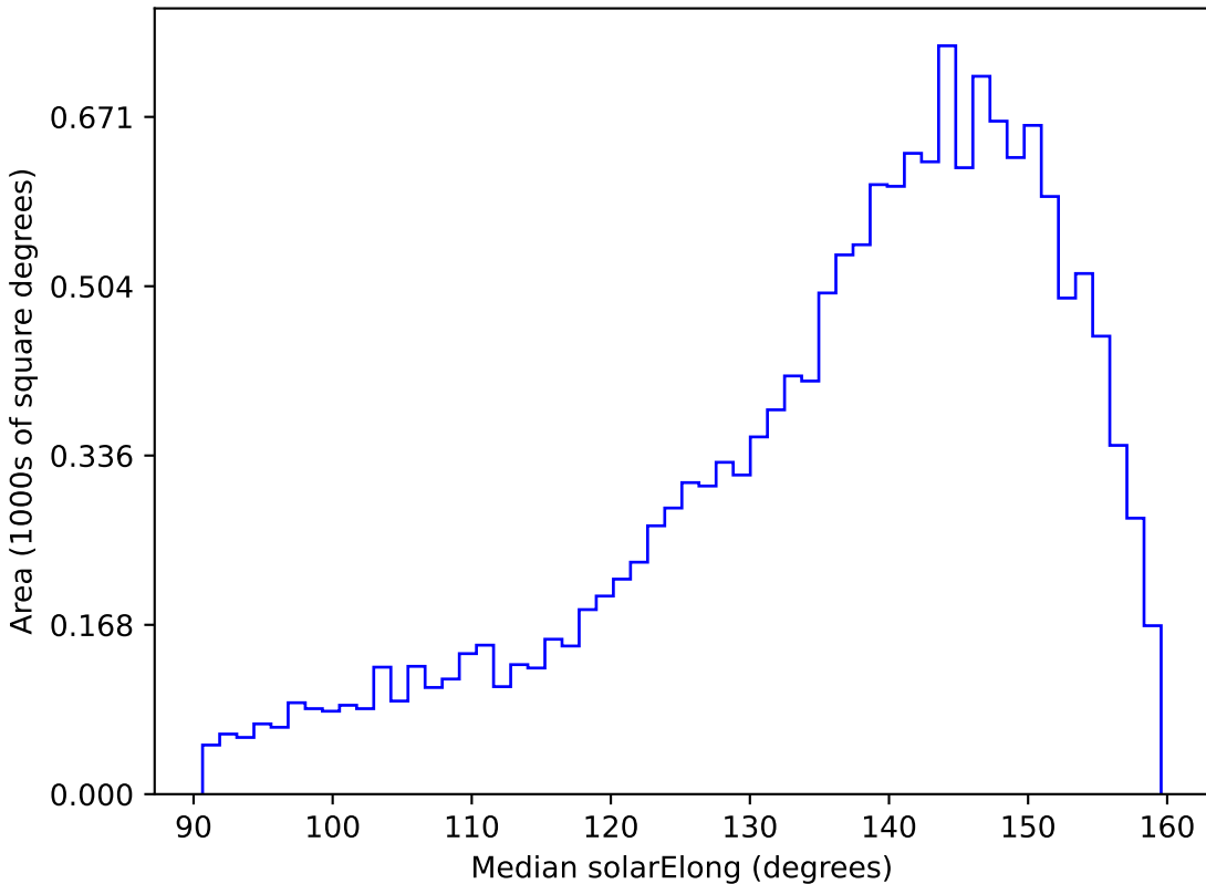
baseline_v3.0_10yrs WFD g band: Median solarElong
