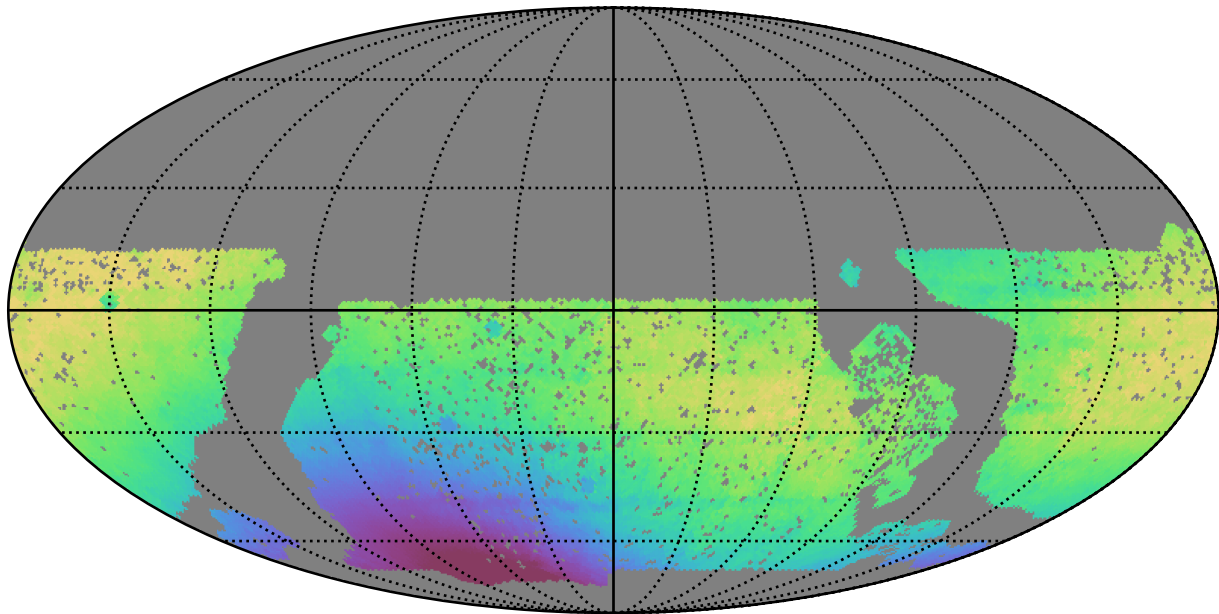
baseline_v3.0_10yrs WFD all bands: Median solarElong
