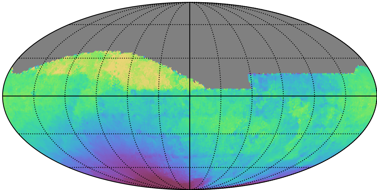
baseline_v3.0_10yrs All sky z band: Median solarElong
