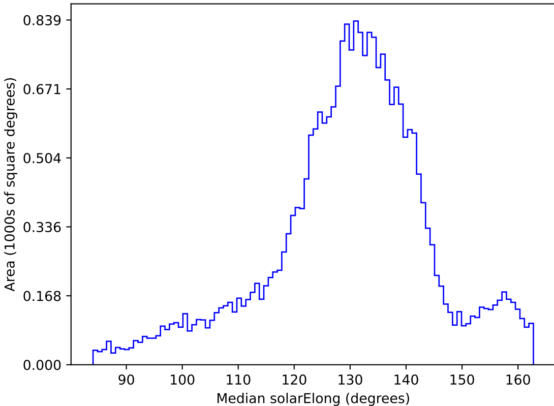
baseline_v3.0_10yrs All sky z band: Median solarElong
