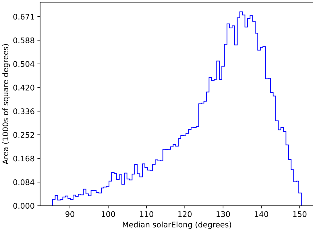
baseline_v3.0_10yrs All sky y band: Median solarElong
