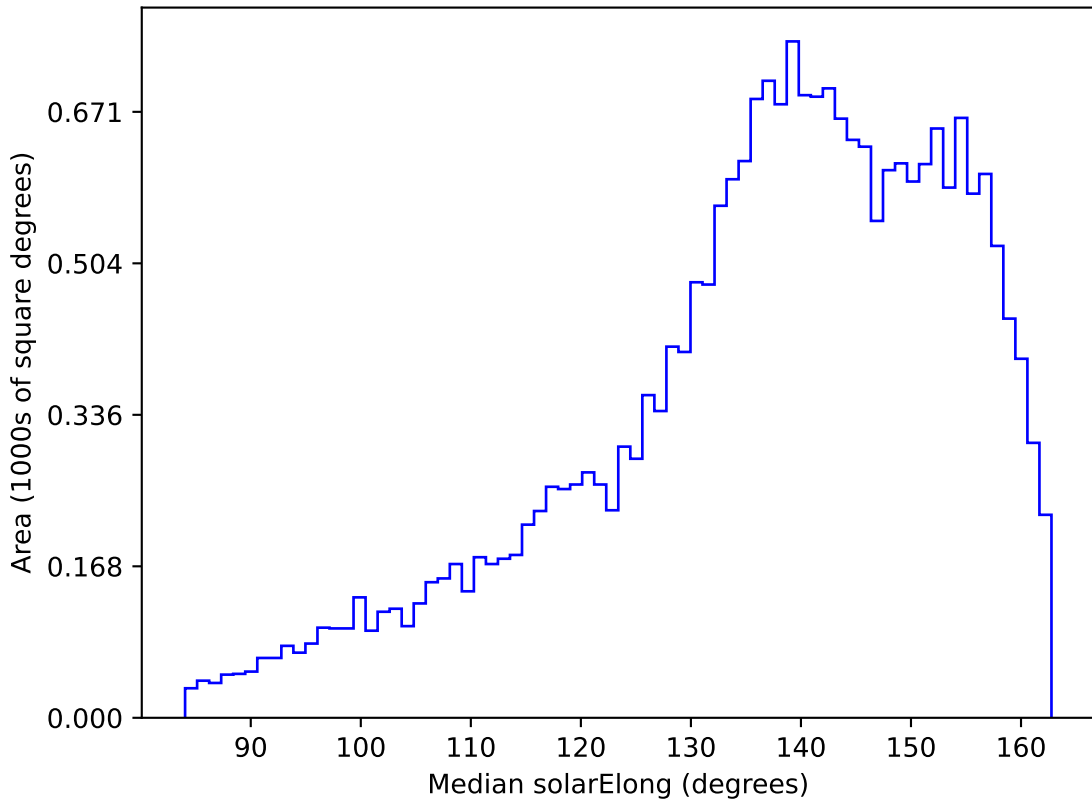
baseline_v3.0_10yrs All sky u band: Median solarElong
