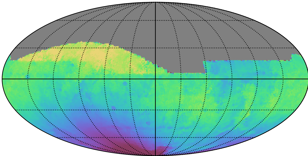
baseline_v3.0_10yrs All sky r band: Median solarElong
