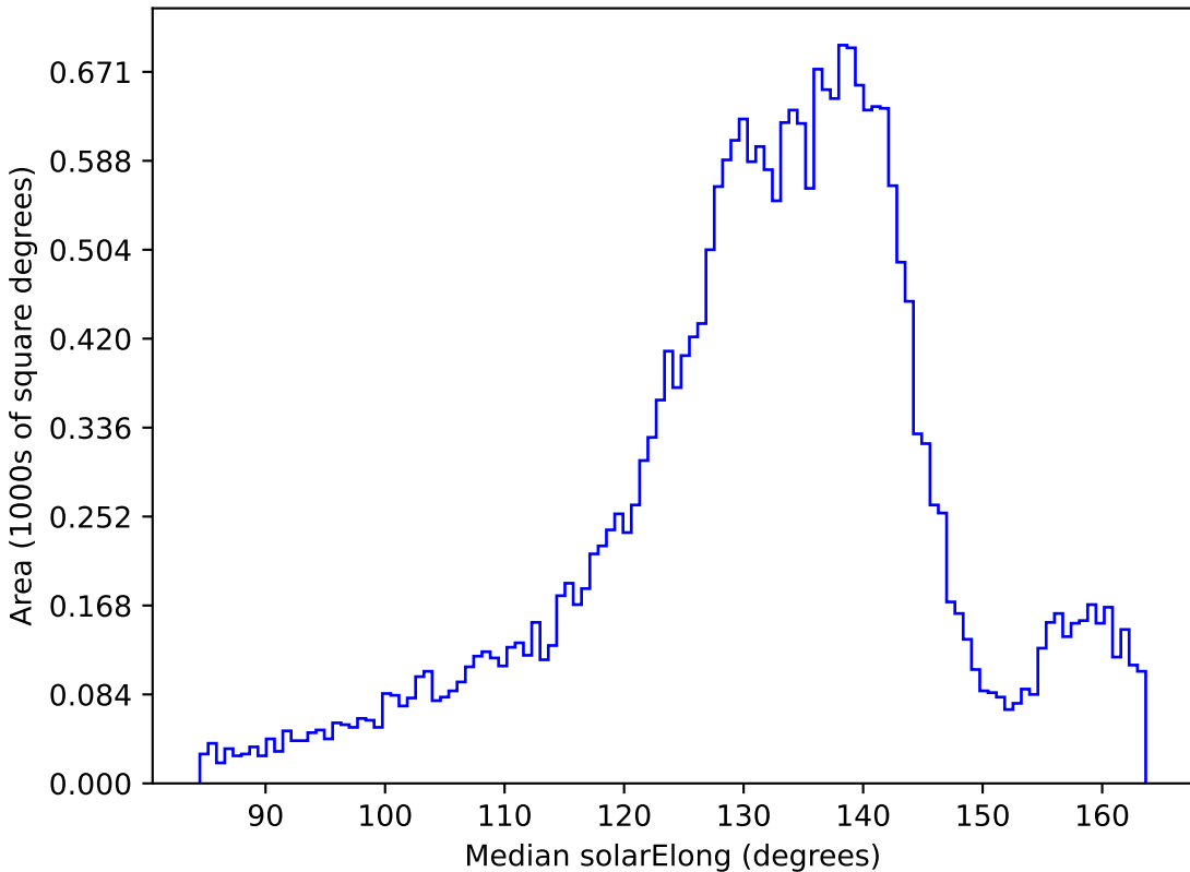
baseline_v3.0_10yrs All sky r band: Median solarElong
