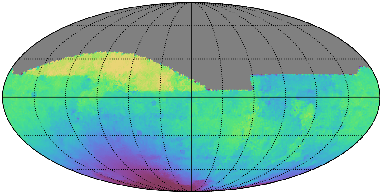
baseline_v3.0_10yrs All sky i band: Median solarElong
