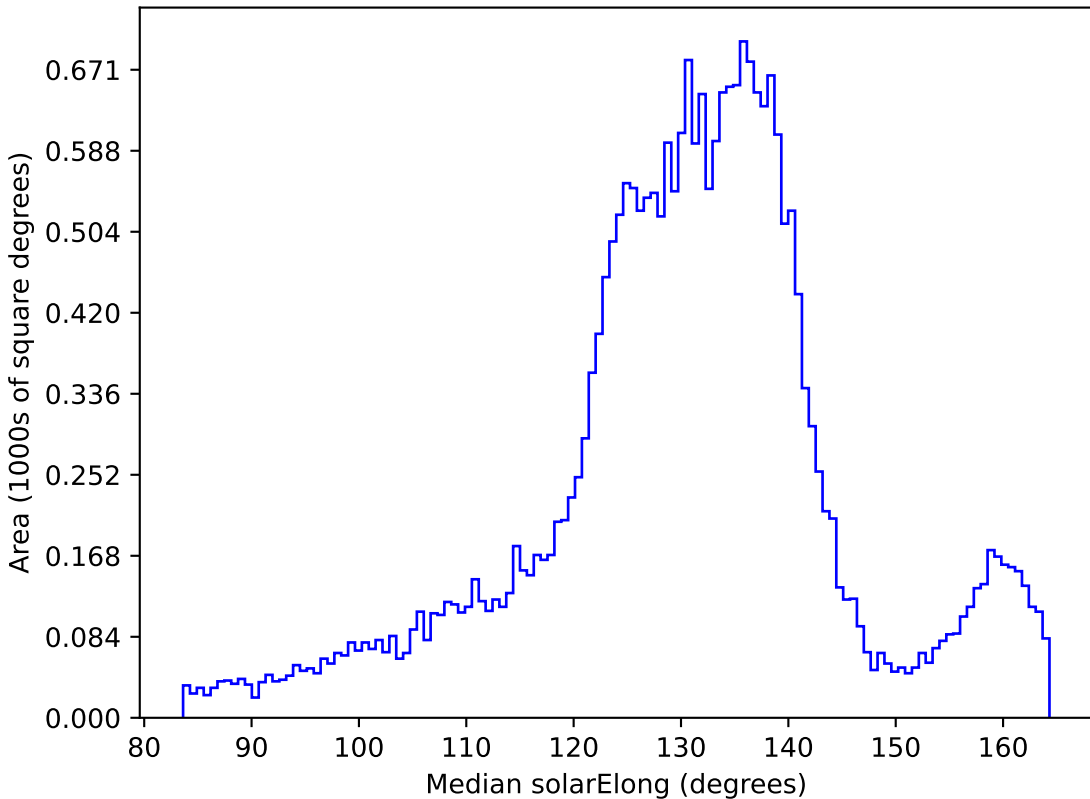
baseline_v3.0_10yrs All sky i band: Median solarElong
