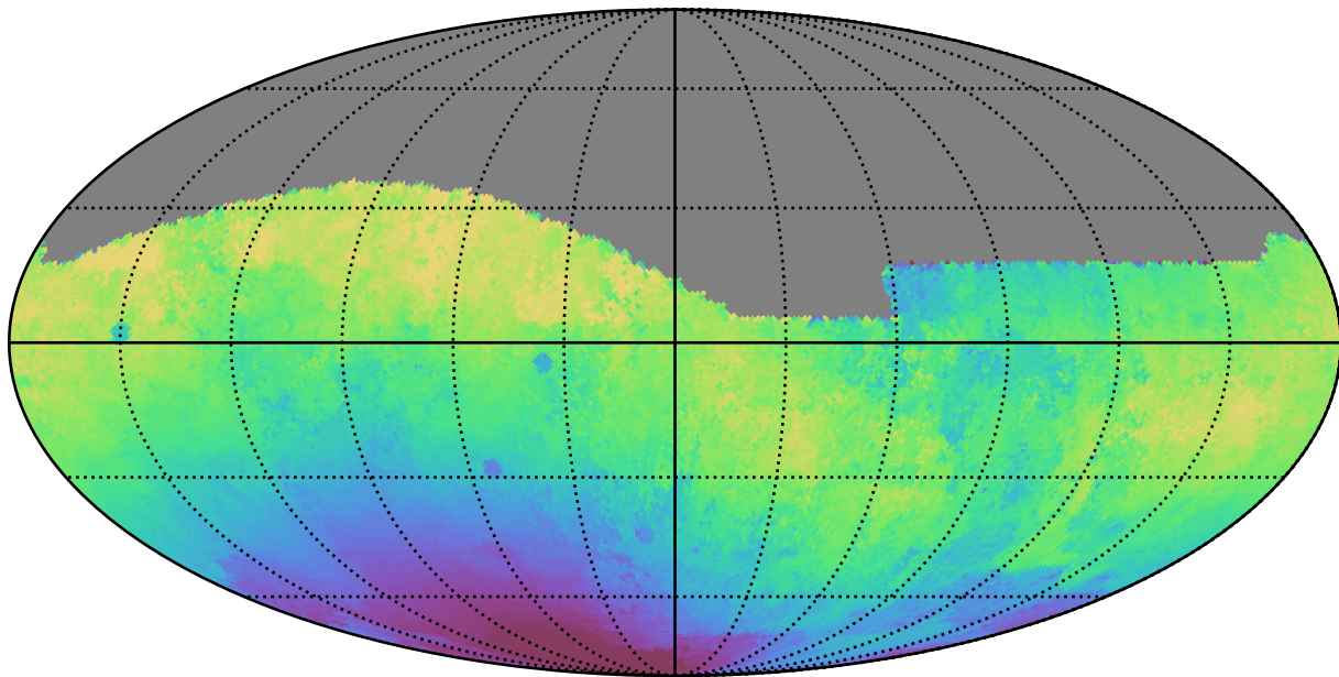
baseline_v3.0_10yrs All sky g band: Median solarElong
