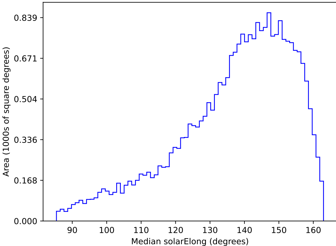
baseline_v3.0_10yrs All sky g band: Median solarElong
