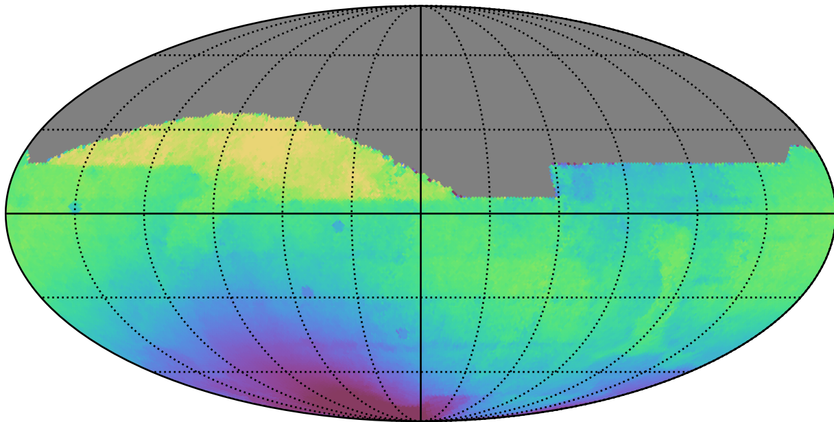
baseline_v3.0_10yrs All sky all bands: Median solarElong
