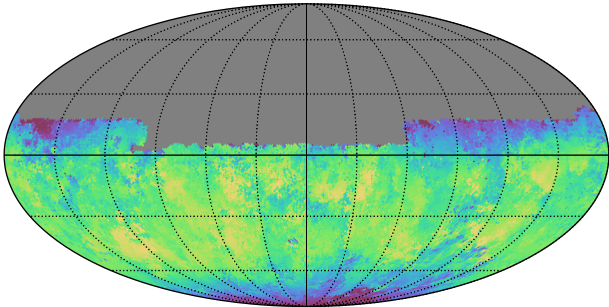
baseline_v3.0_10yrs Yr 1 y band: Median skyBrightness
