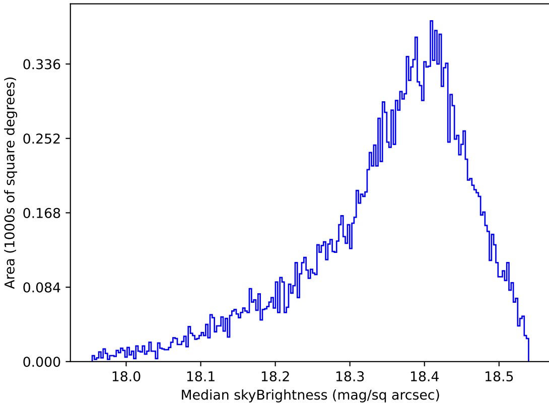
baseline_v3.0_10yrs Yr 1 y band: Median skyBrightness
