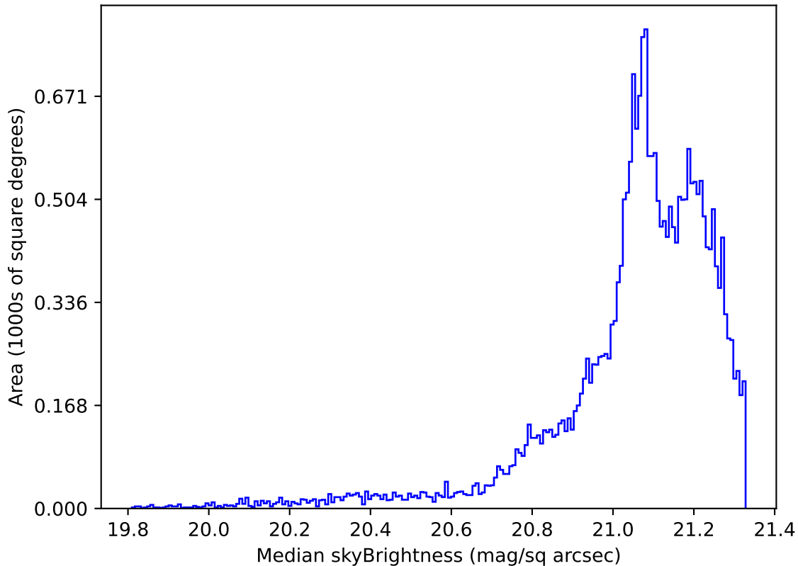
baseline_v3.0_10yrs Yr 1 r band: Median skyBrightness
