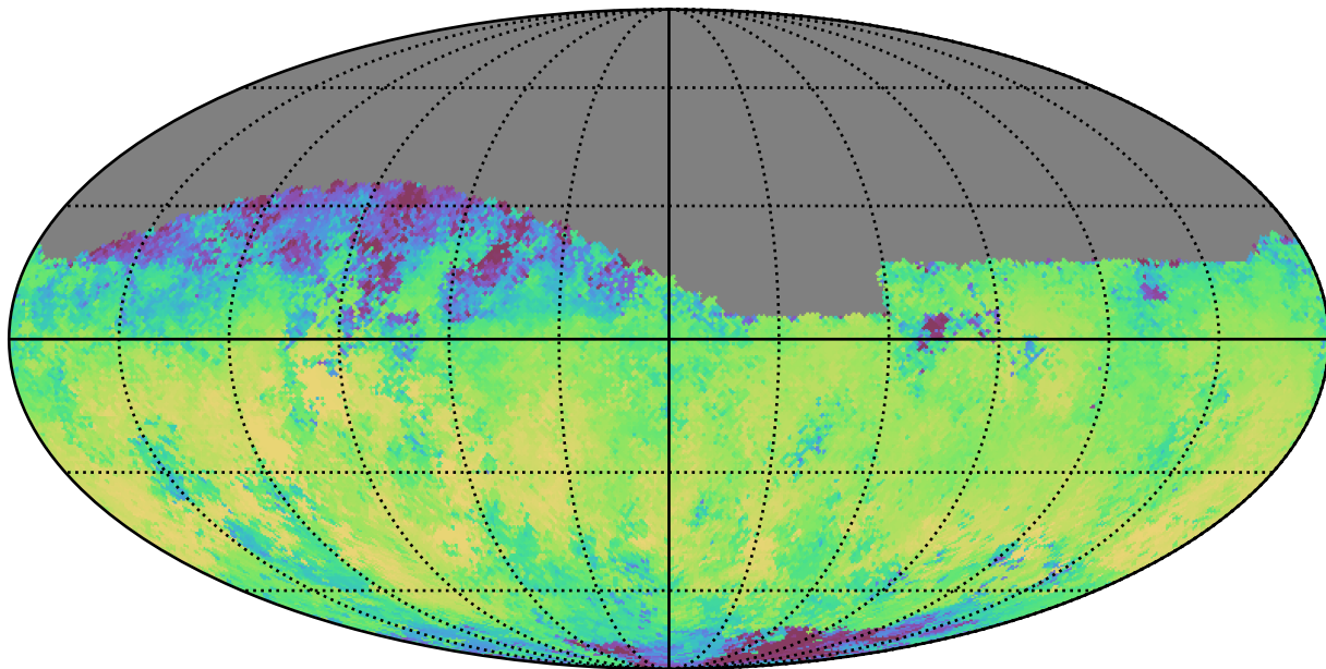
baseline_v3.0_10yrs Yr 1 i band: Median skyBrightness
