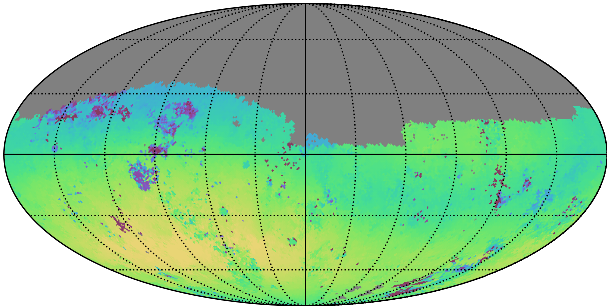
baseline_v3.0_10yrs Yr 1 g band: Median skyBrightness
