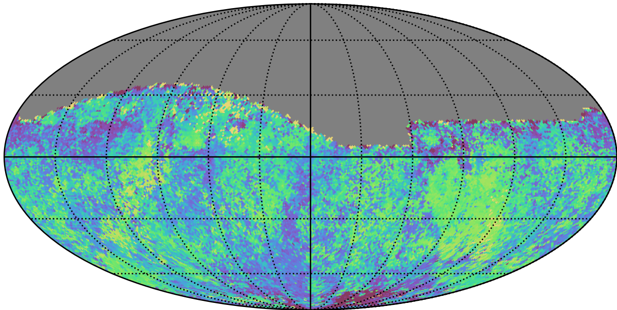
baseline_v3.0_10yrs Yr 1 all bands: Median skyBrightness
