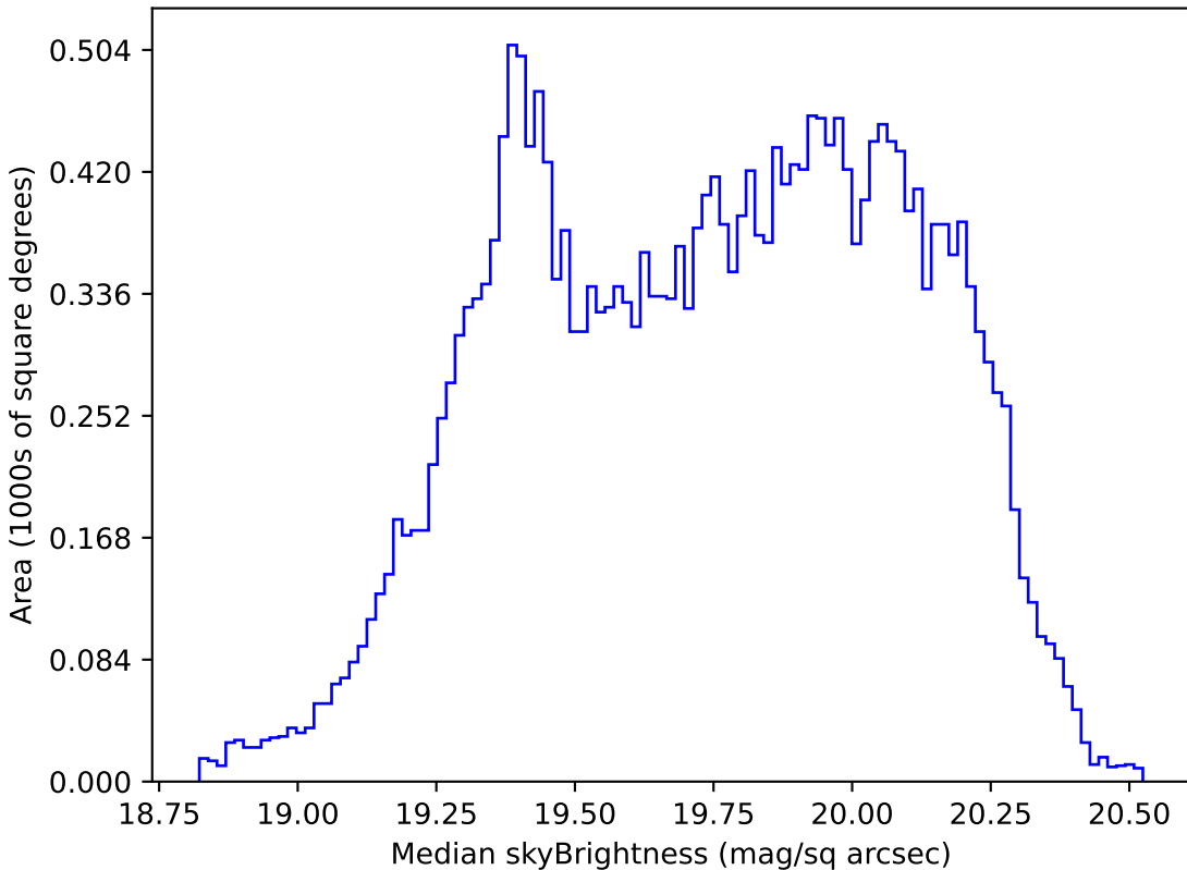
baseline_v3.0_10yrs Yr 1 all bands: Median skyBrightness
