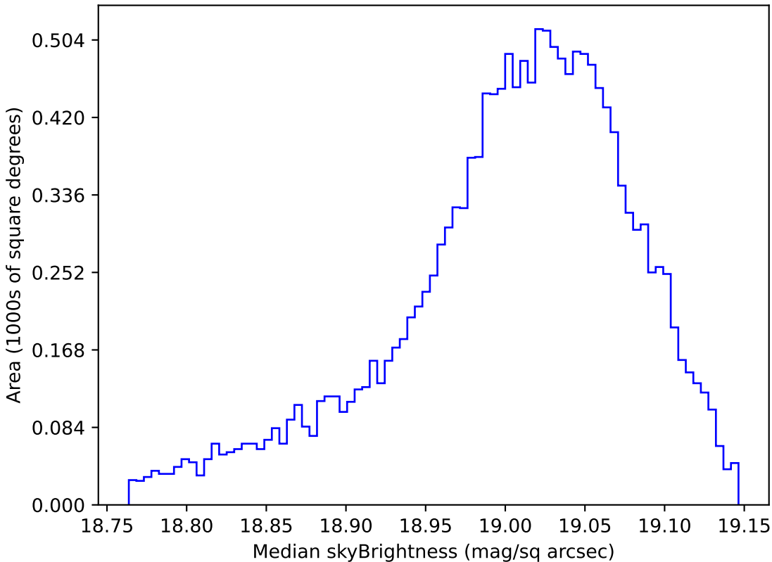
baseline_v3.0_10yrs WFD z band: Median skyBrightness
