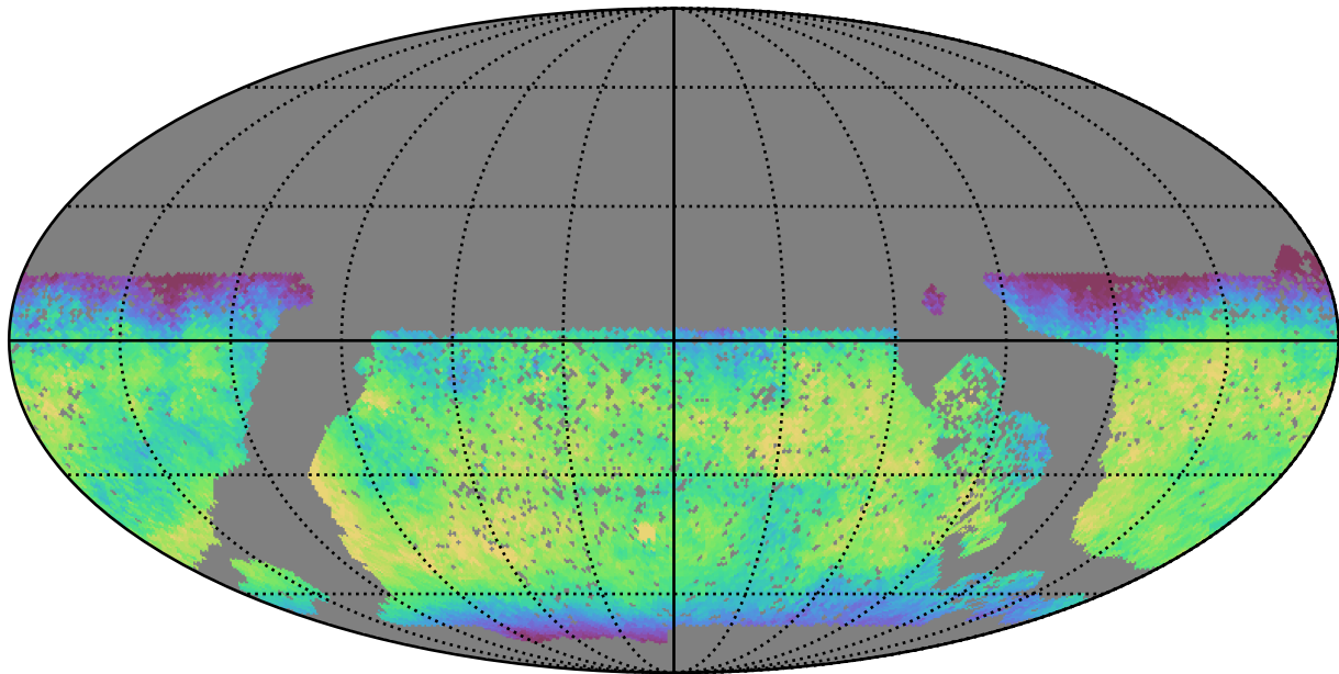
baseline_v3.0_10yrs WFD y band: Median skyBrightness
