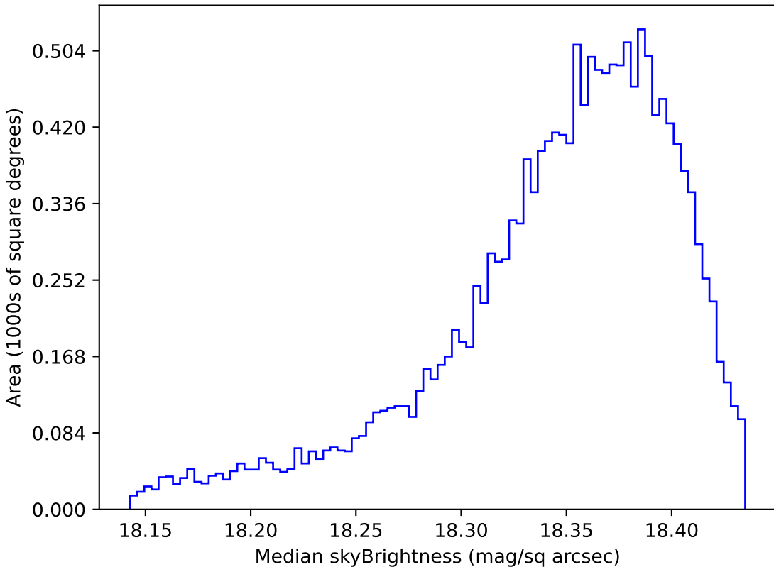
baseline_v3.0_10yrs WFD y band: Median skyBrightness
