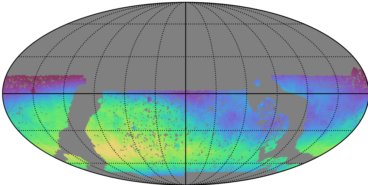
baseline_v3.0_10yrs WFD u band: Median skyBrightness
