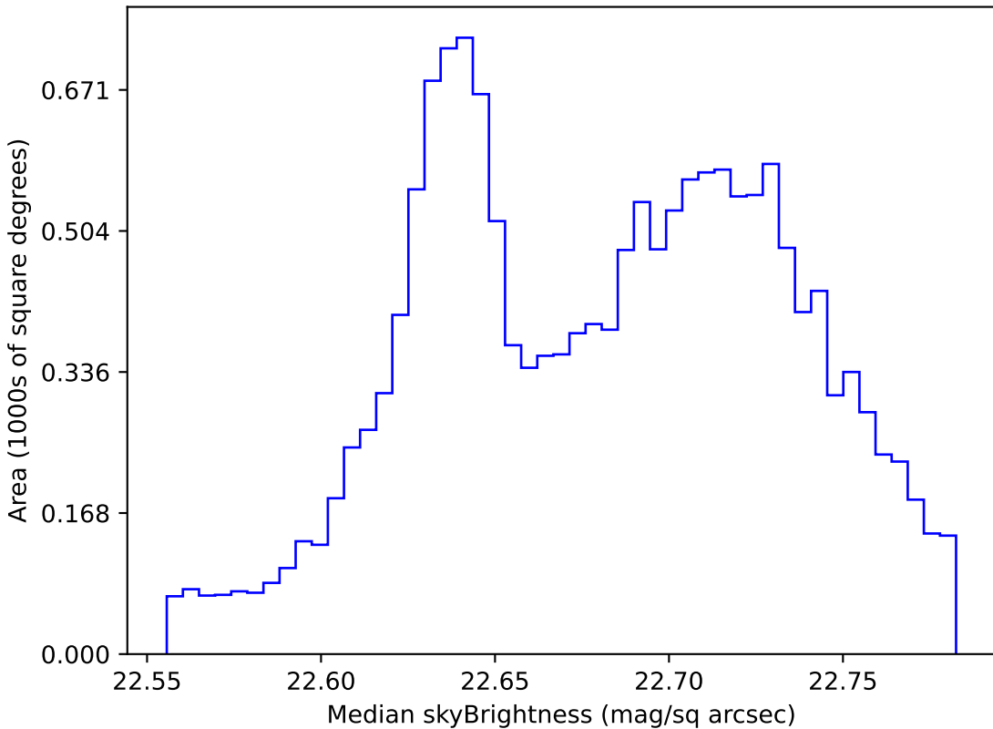
baseline_v3.0_10yrs WFD u band: Median skyBrightness
