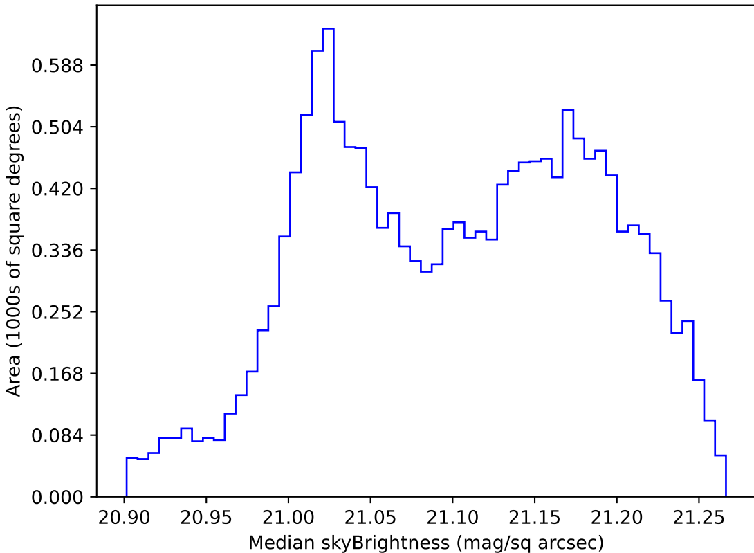
baseline_v3.0_10yrs WFD r band: Median skyBrightness
