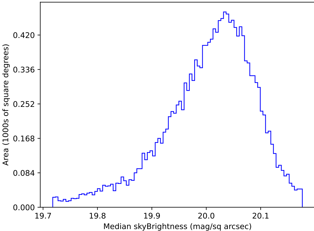
baseline_v3.0_10yrs WFD i band: Median skyBrightness
