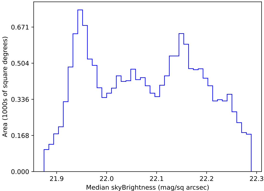
baseline_v3.0_10yrs WFD g band: Median skyBrightness
